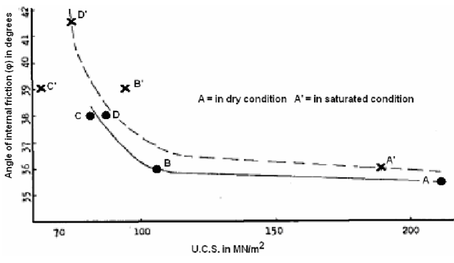
Figure 14. Relationship between the angle of internal friction and the unconfined compressive strength of all grades.
